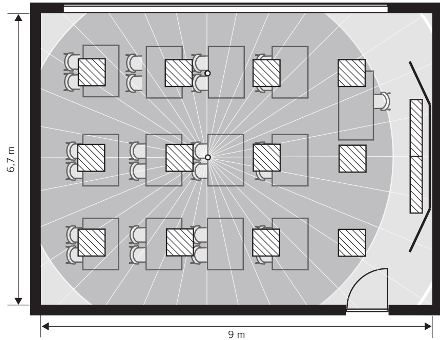
▲ Planning example of installation of classroom set 1 in a typical classroom approximately 60 m 2 in size. Room height 3 m, planning criterion 500 lux (suitable for adult education) at a working level of 0.75 m.
