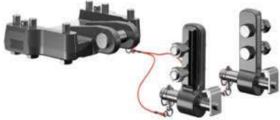
Bottom hitch attachment parts Basic (A179)
